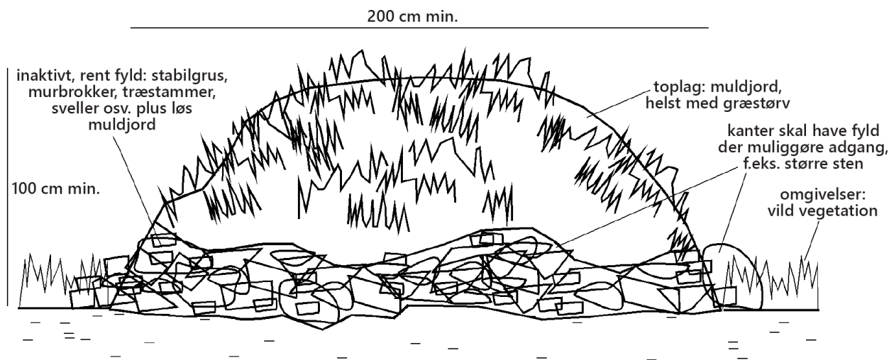
Figur 7: Opbygning af overvintringsted for firben. Kilde: Great crested newt mitigation guidelines 2001.
